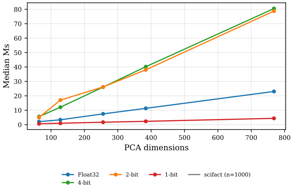
NumPy pairwise distance
