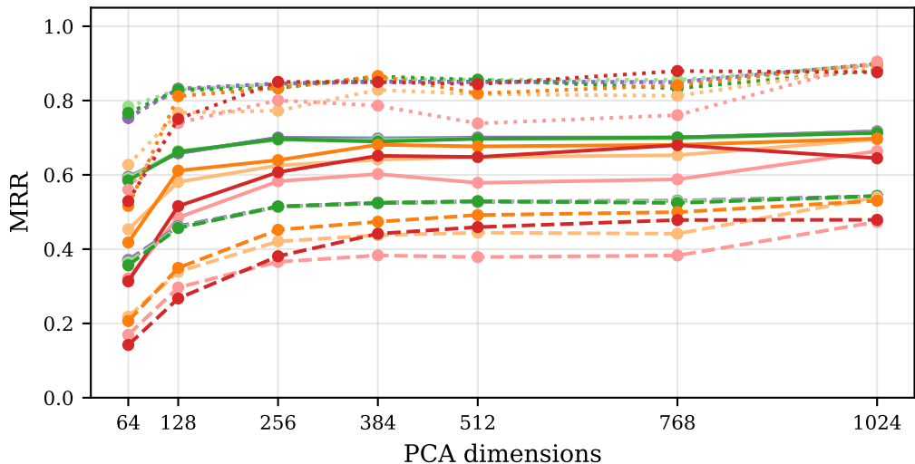
Retrieval MRR by Dimension
