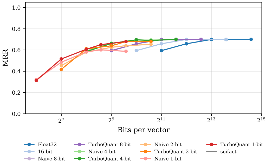
Retrieval MRR vs. Compression
