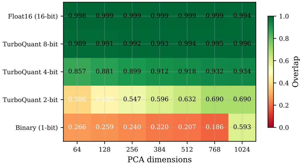
fiqa — Overlap (k=20)
