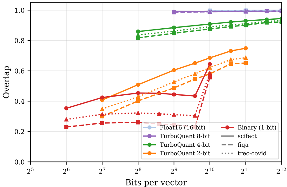
Overlap vs. Compression (k=5)
