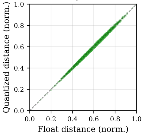
TurboQuant 4-bit
