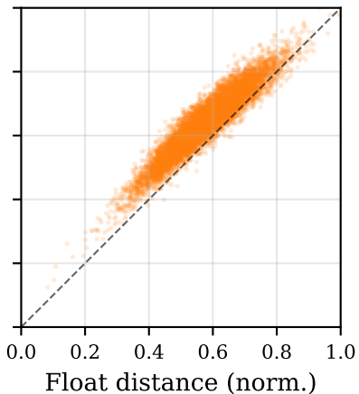
TurboQuant 2-bit
