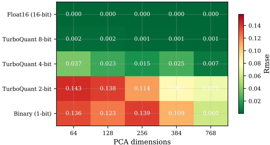
scifact — RMSE
