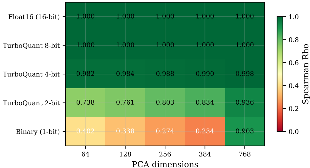
scifact — Spearman \rho
