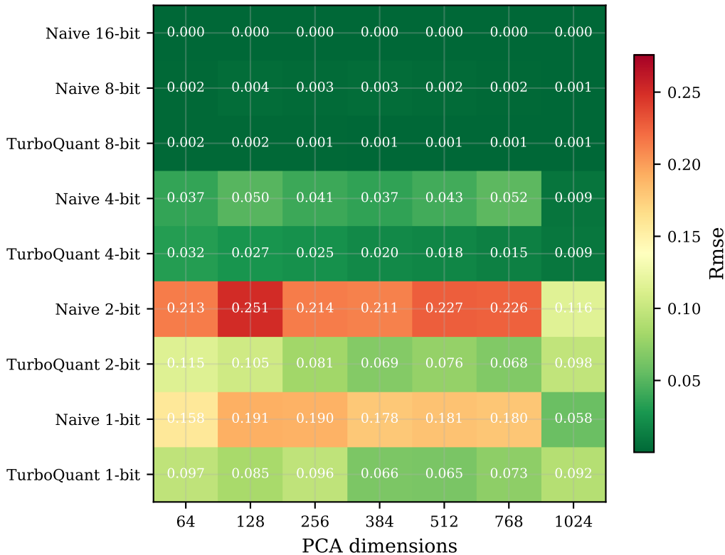
fiqua — RMSE
