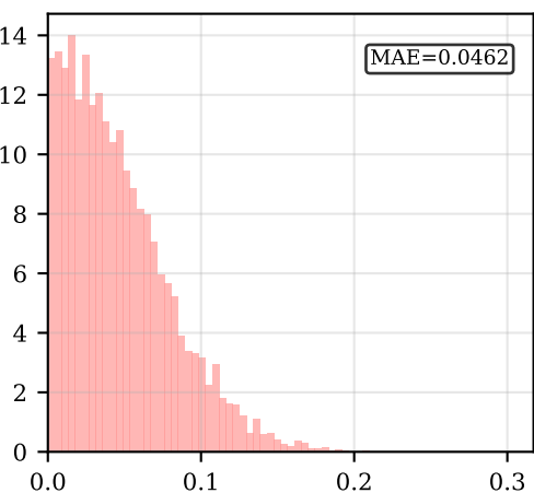
Naive 1-bit
