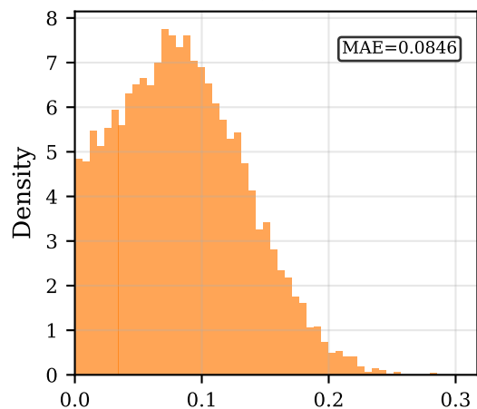
TurboQuant 2-bit
