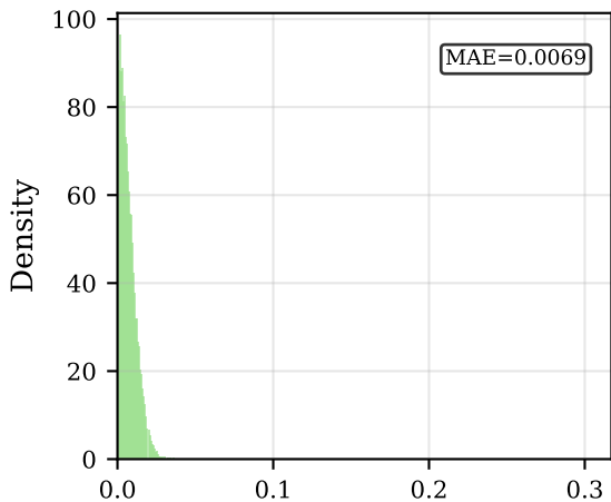
TurboQuant 2-bit
