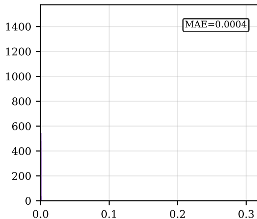
Naive 2-bit
