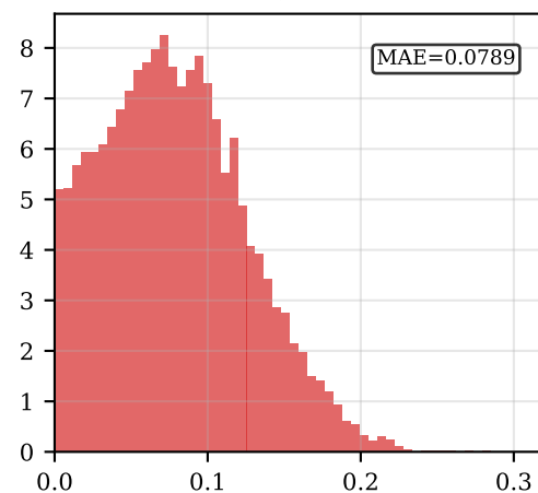
TurboQuant 1-bit
