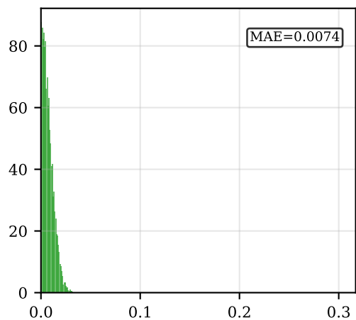
Naive 1-bit
