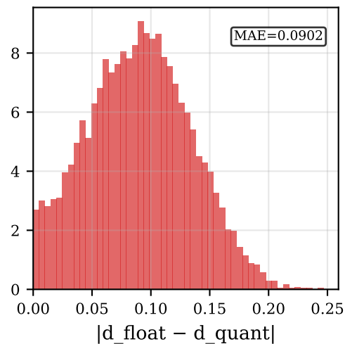
TurboQuant 1-bit
