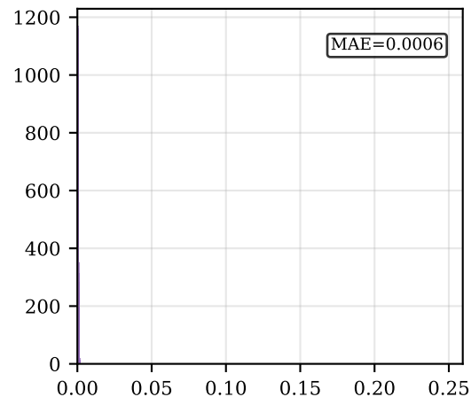
Naive 2-bit
