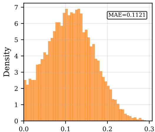
TurboQuant 2-bit
