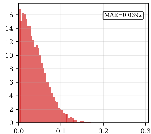
TurboQuant 1-bit
