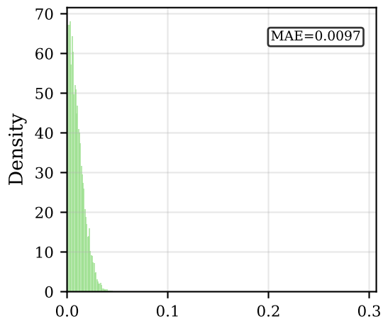
TurboQuant 2-bit
