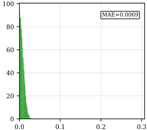
Naive 1-bit
