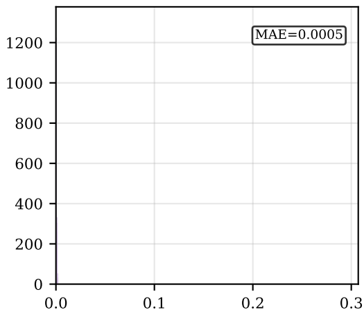
TurboQuant 4-bit
