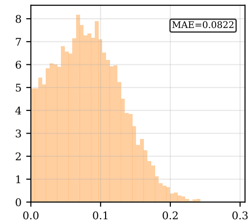
TurboQuant 1-bit
