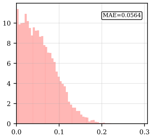
Naive 1-bit
