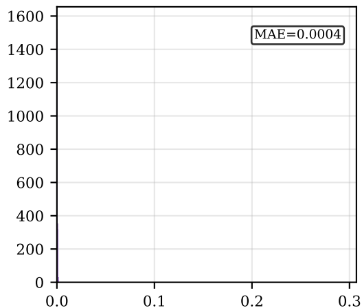
Naive 2-bit
