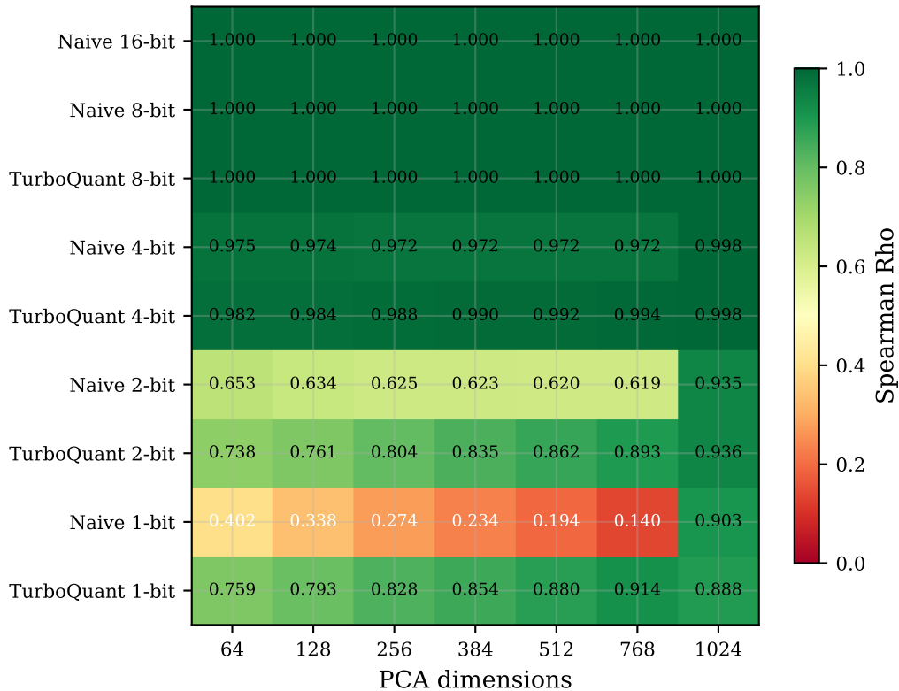
scifact — Spearman \rho
