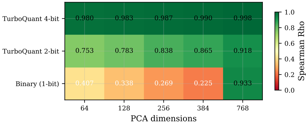
fiqa — Spearman \rho
