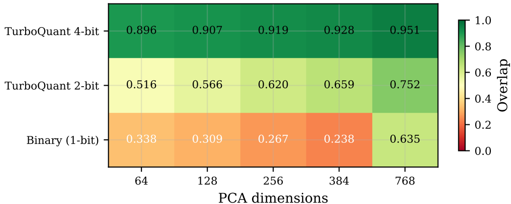
scifact — Overlap (k=100)
