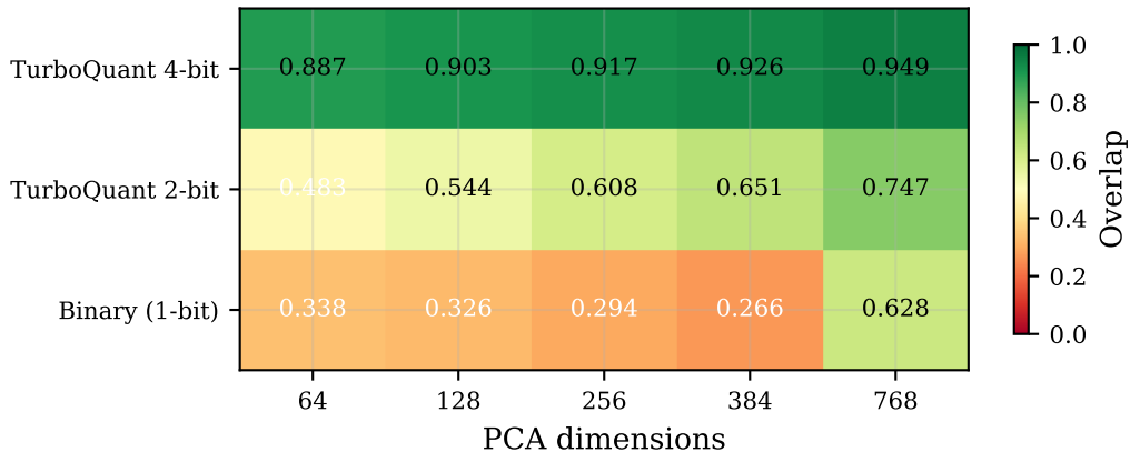
scifact — Overlap (k=50)
