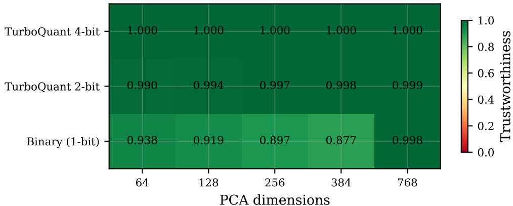
fiqa — Trustworthiness (k=10)
