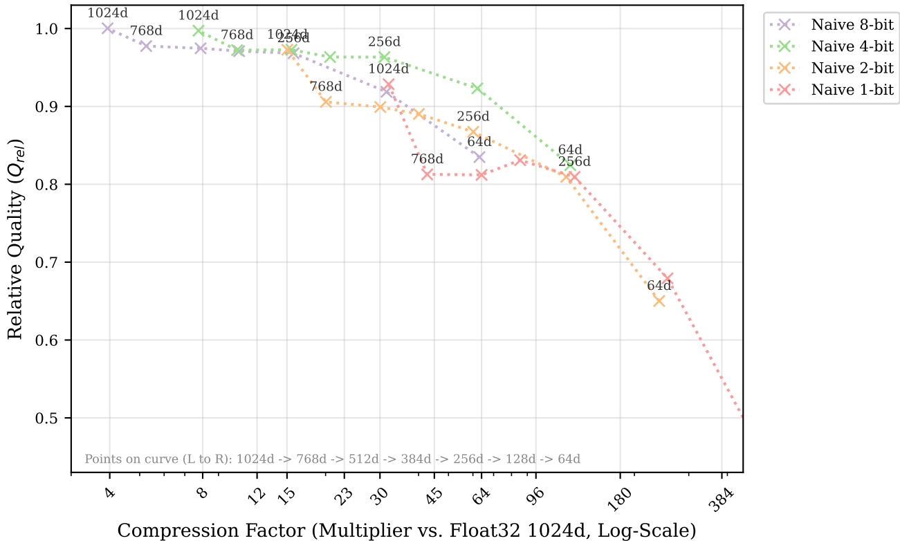
Quality vs. Compression Factor (Naive Only)
