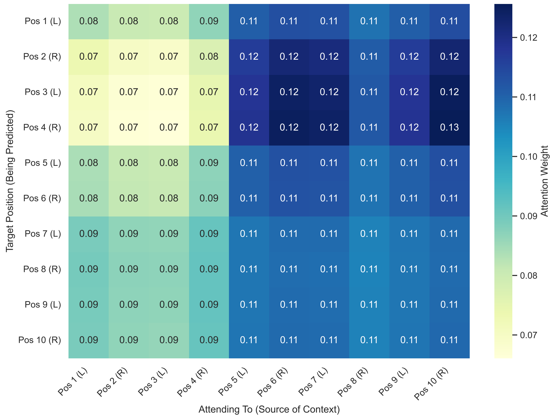
XPA Cross-Positional Attention Weights (How layout slots influence each other)
