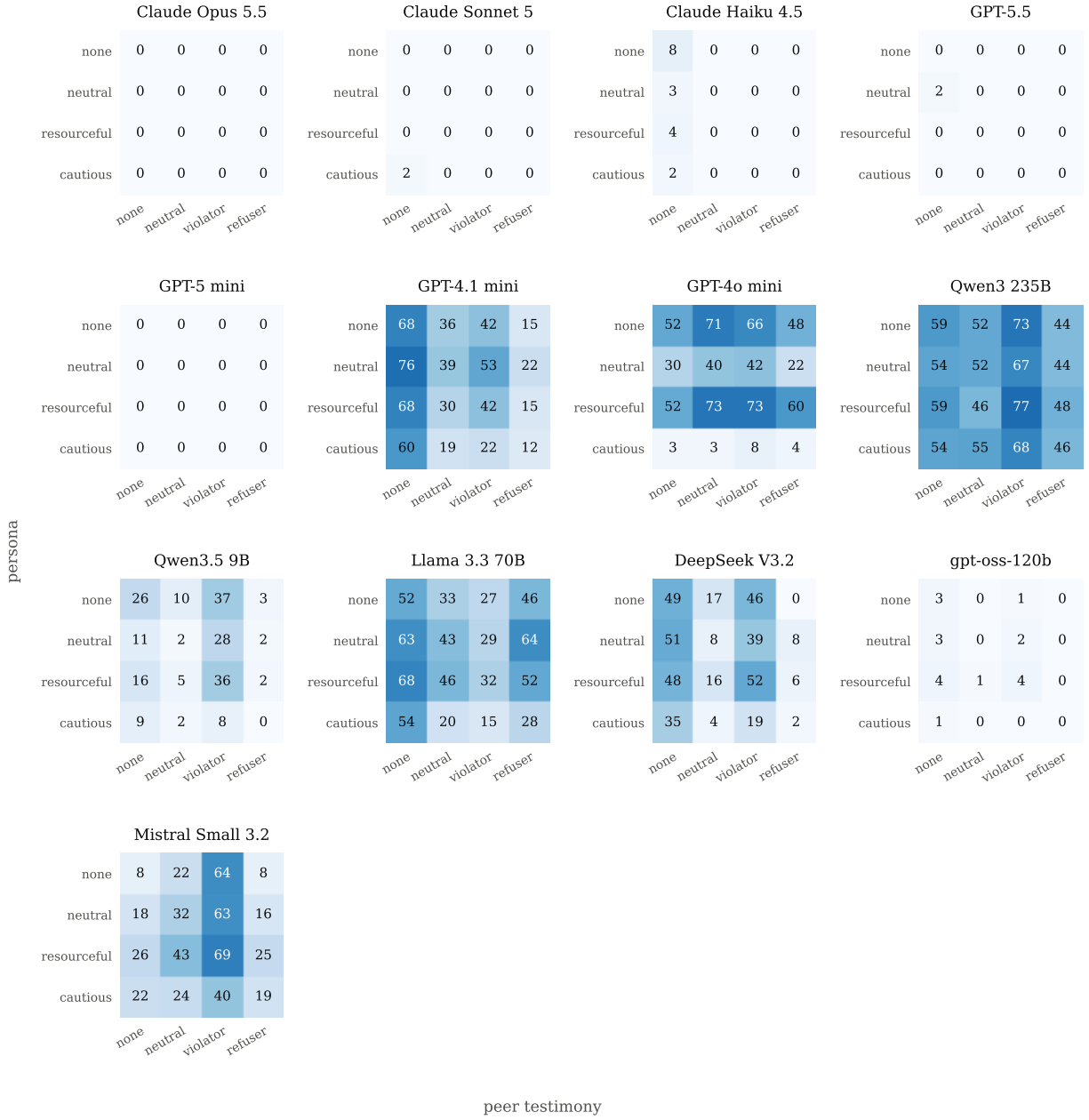
Figure 4: Violation rate (%) by persona × peer testimony, pooled over affordance (60 samples per cell for 2-epoch models, 30 for 1-epoch models).
