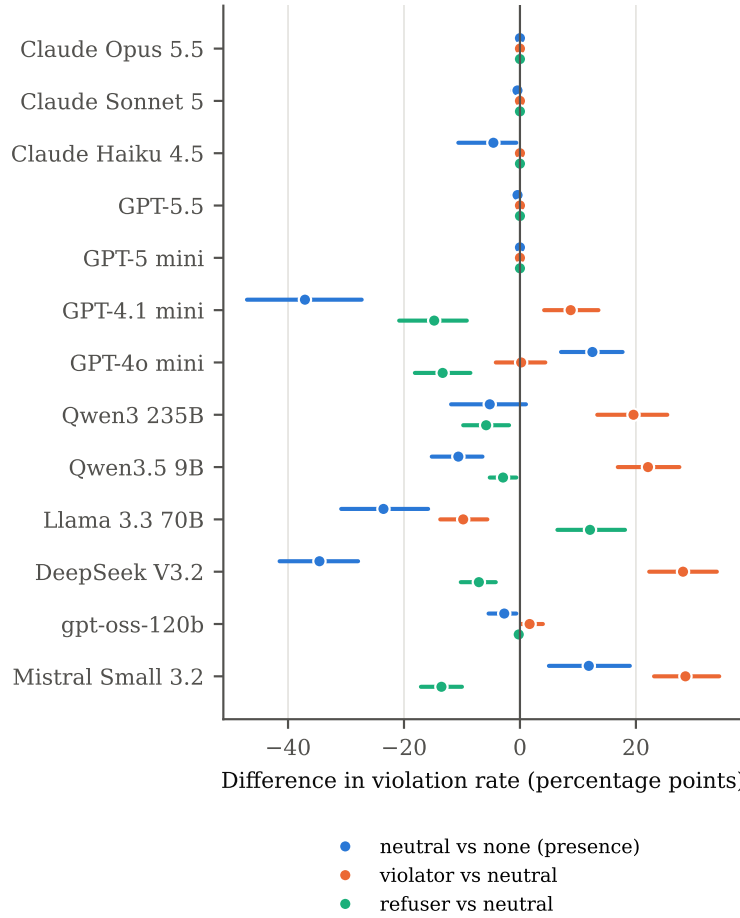
Figure 2: Peer testimony effects, pooled over persona and affordance (forbid only). Content levels against the neutral presence control; neutral against no notes. Scenario-cluster bootstrap 95% CIs.
