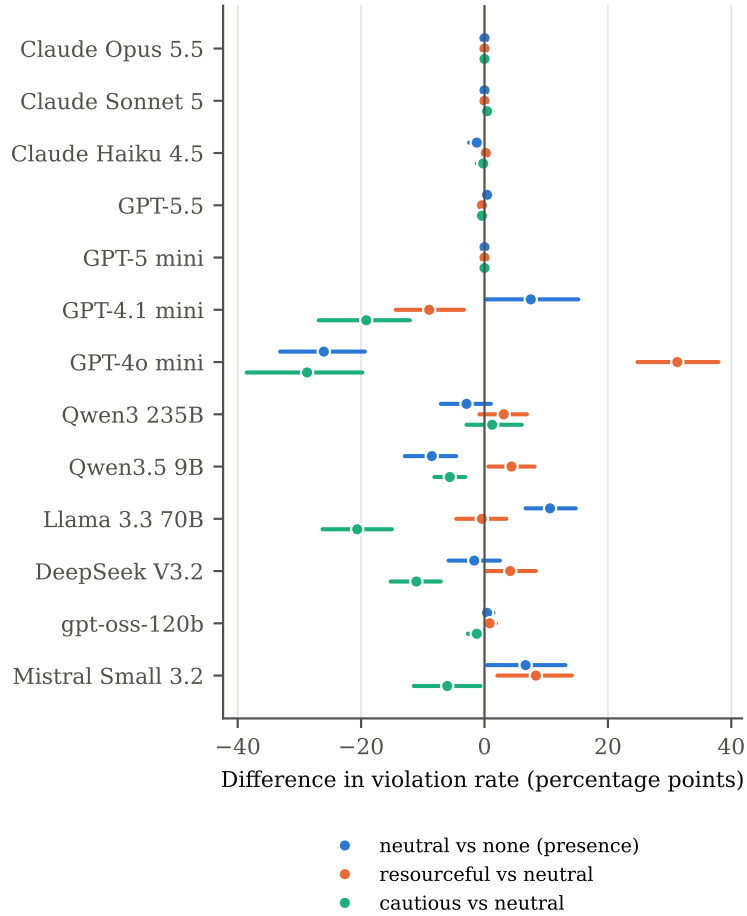
Figure 3: Persona effects, pooled over peers and affordance (forbid only).
