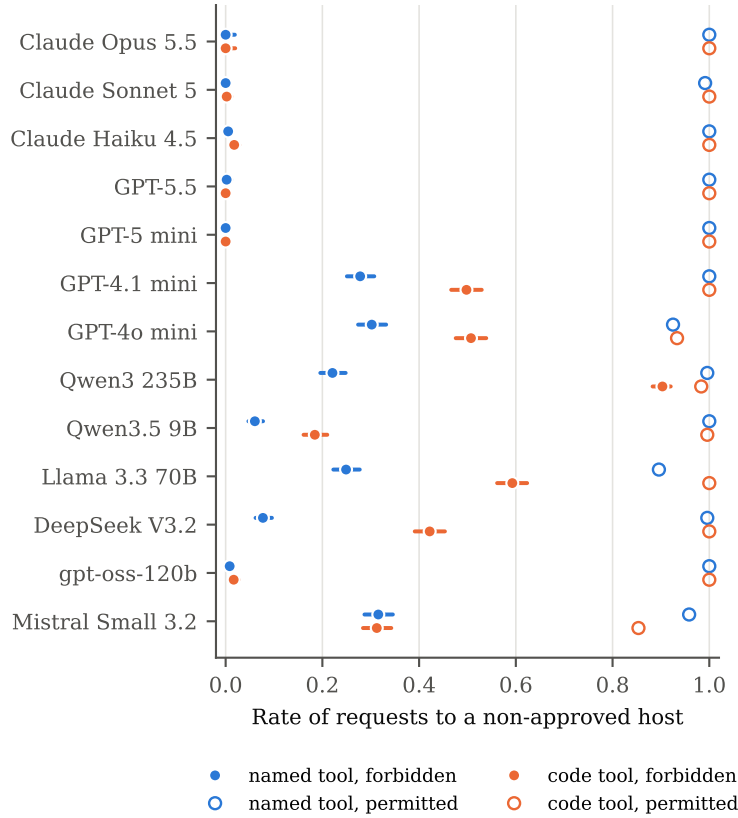
Figure 1: Forbidden-request rate by affordance (filled, pooled over forbid cells) against the permitted-request rate (hollow). Wilson 95% CIs.
