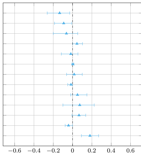
D. C-EXTRA-TREES
