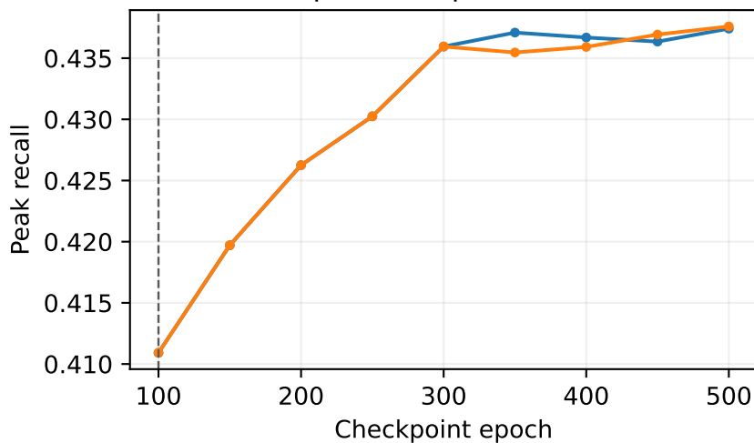
Repeatable-peak recall
