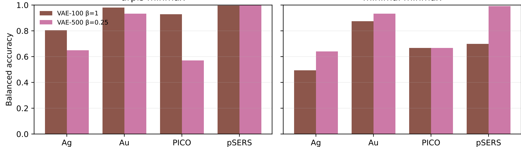
arpls minmax
