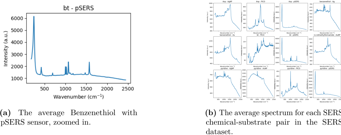
Figure 10: Average spectrum for the SERS data. A distinctive, and in some cases, dominant peak at around 300\text{cm}^{-1} can be observed.
