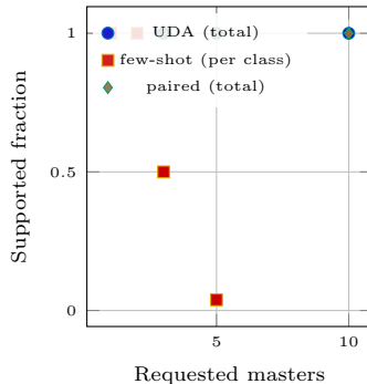
Target-access feasibility
