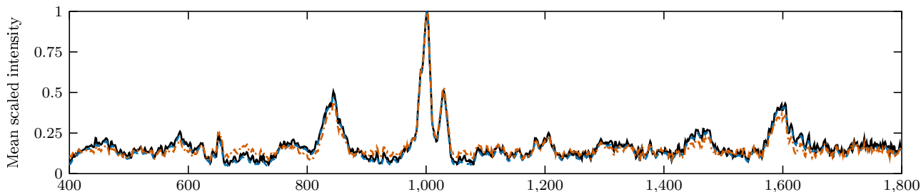
B. benzyl_fentanyl (physical masters: 4; stored spectra: 4)
