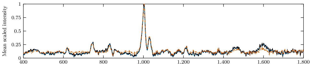
C. blank (physical masters: 8; stored spectra: 9)
