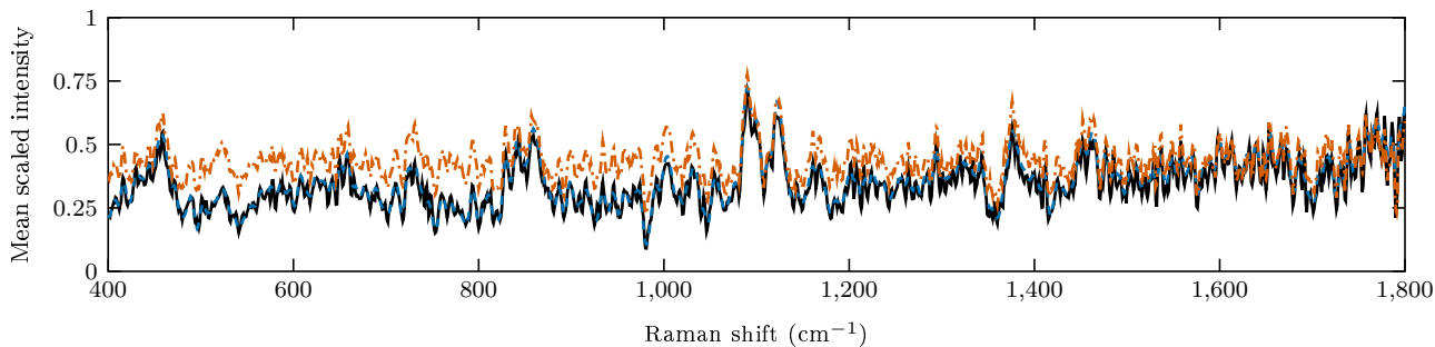
C. blank (physical masters: 8; stored spectra: 9)
