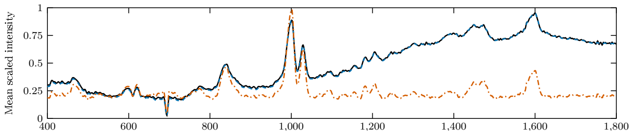
A. 4_ANPP (physical masters: 3; stored spectra: 3)
