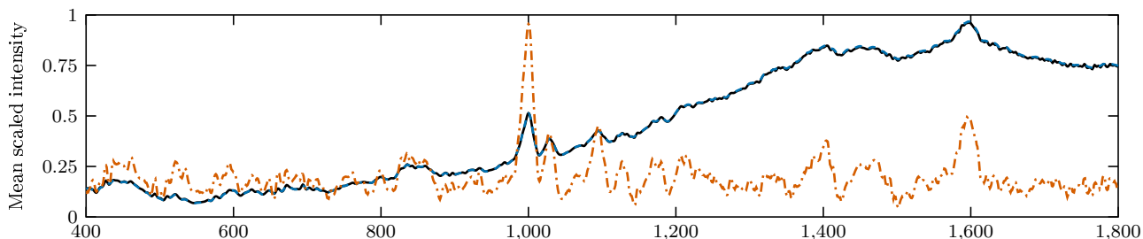
C. benzyl_fentanyl (physical masters: 7; stored spectra: 11)
