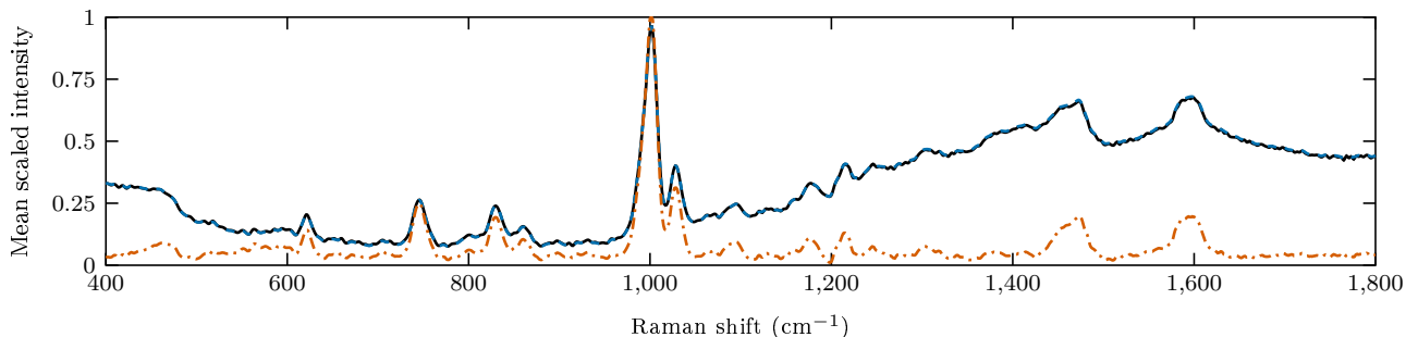
C. benzyl_fentanyl (physical masters: 7; stored spectra: 11)
