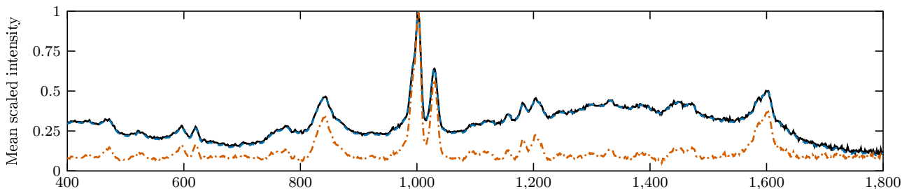
A. 4_ANPP (physical masters: 4; stored spectra: 12)
