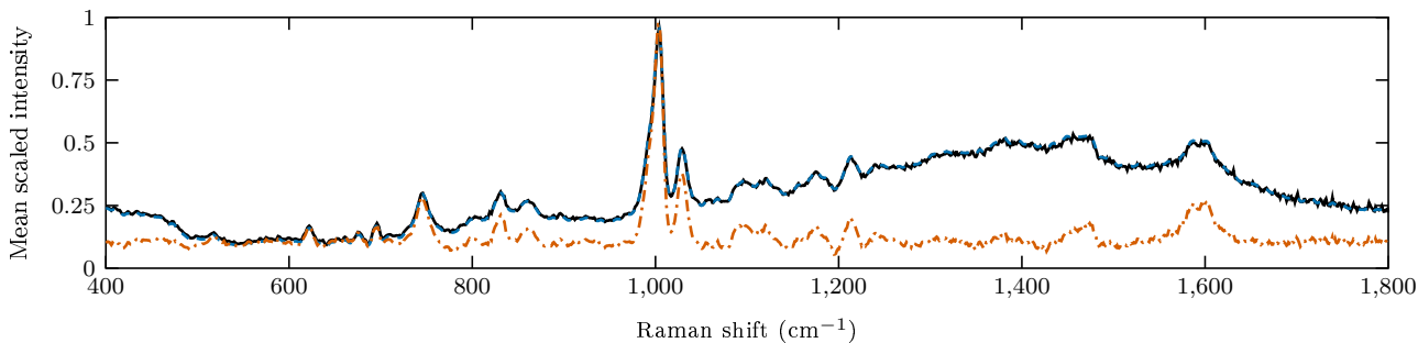
C. benzyl_fentanyl (physical masters: 10; stored spectra: 24)
