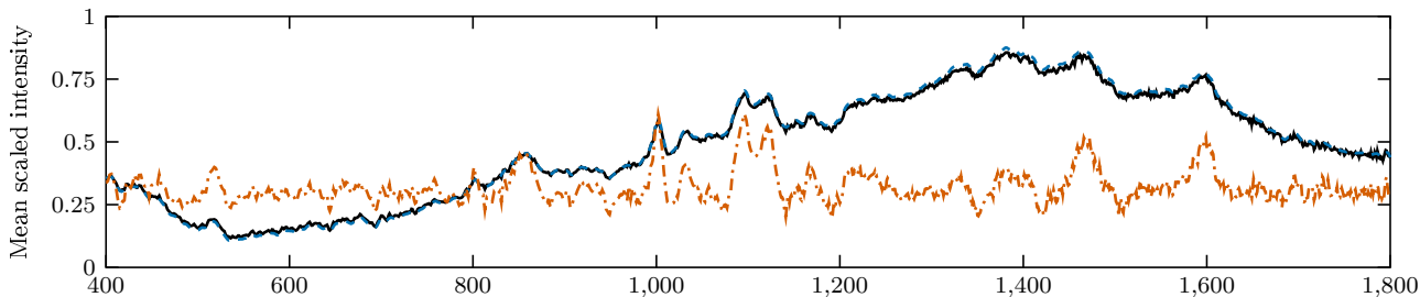
C. benzyl_fentanyl (physical masters: 10; stored spectra: 24)
