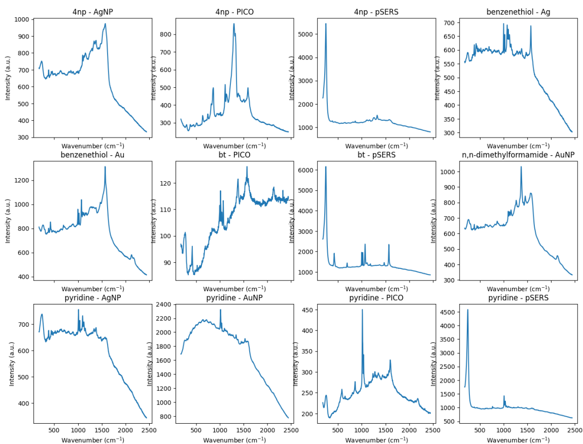
Figure 10: Plots of the average spectrum for each chemical-substrate pair.
