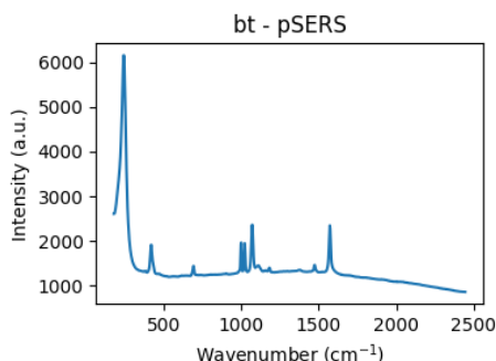
(a) The average Benzenethiol with pSERS sensor, zoomed in.
