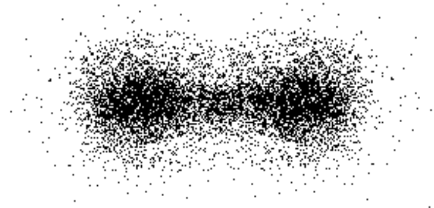
Bonding
