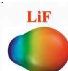
\text{Li}^+ \text{F}^-
