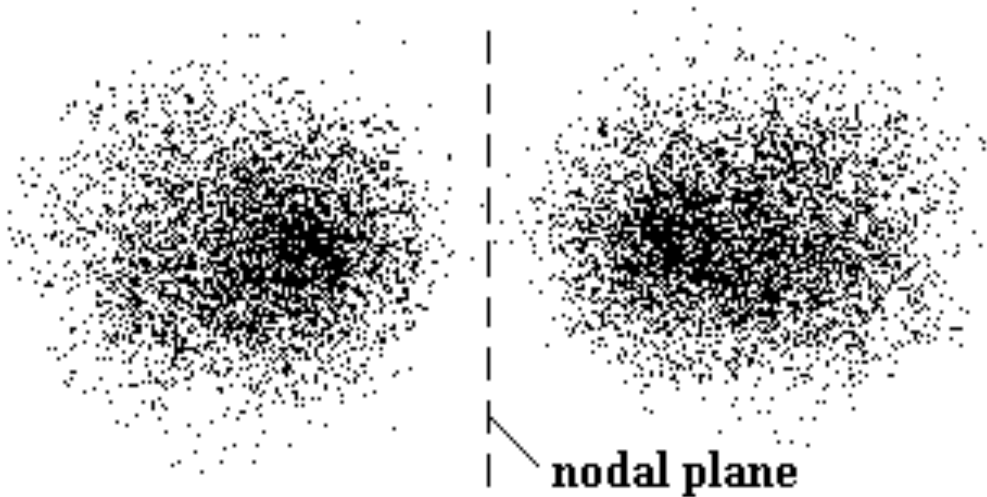
Anti-Bonding
