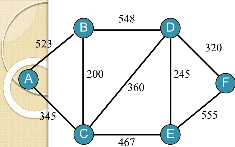
City Network
