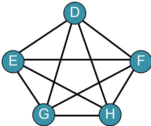
Undirected graph
