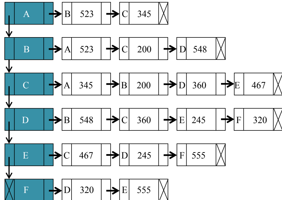
Adjacency List
