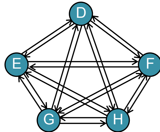
Directed graph
