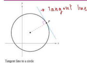
Tangent line to a circle
