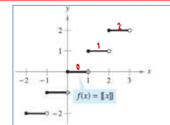
The greatest integer function is not differentiable at x = 0 , because it is not continuous at x = 0 .
