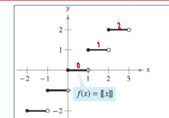
The greatest integer function is not differentiable at x = 0 , because it is not continuous at x = 0 .
