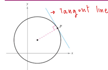
Tangent line to a circle
