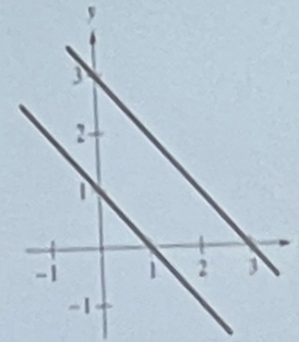
(c) Two parallel lines: x + y = 3 x + y = 1
