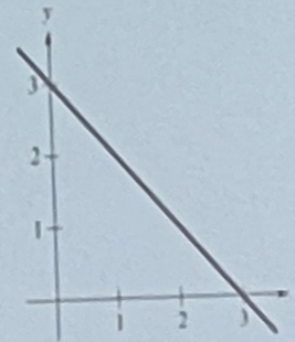
(b) Two coincident lines: x + y = 3 2x + 2y = 6
