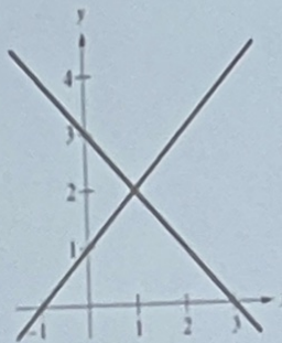
(a) Two intersecting lines: x + y = 3 x - y = -1
