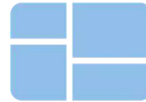
Windows 1.0
