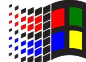
Windows 3.5
