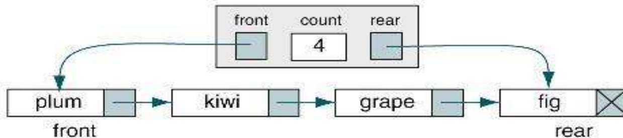
(b) Physical queue
