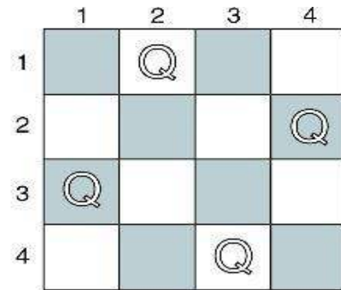
(b) First four queens solution
