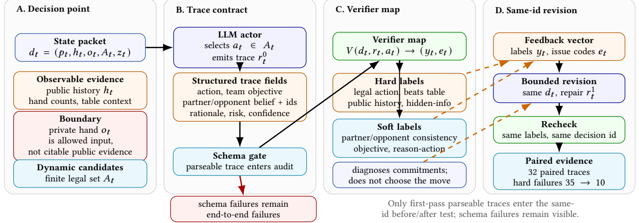
Figure 2: Trace-contract verifier architecture. A decision point is converted into a structured trace with explicit evidence boundaries; the verifier maps the same state, trace, and selected action to labels and issue codes, then supports bounded same-state revision without choosing the action. Paired evidence uses only first-pass parseable traces, while parse failures remain explicit end-to-end reliability failures.
