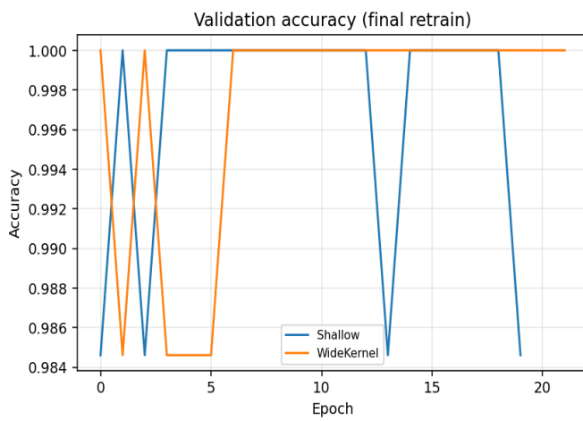
Training curves (final retrain on full training pool)
