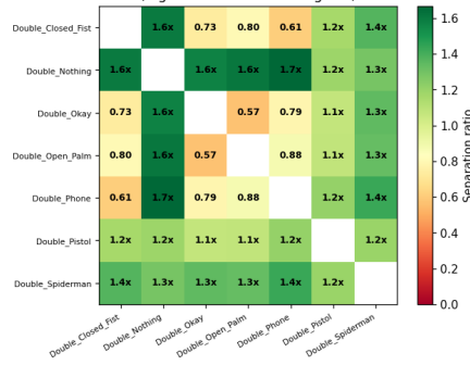
User 11_Mansh — extracted features (stats+fft) Between-class Separation Ratio (higher = easier to distinguish)
