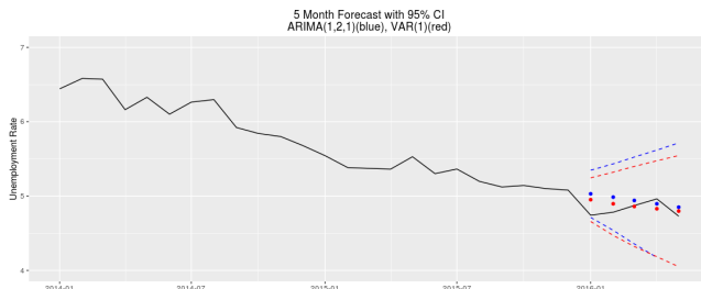
Figure 29: Other plot
