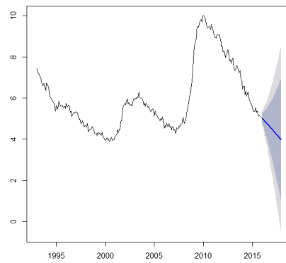
Forecasts from ARIMA(1,2,1)
