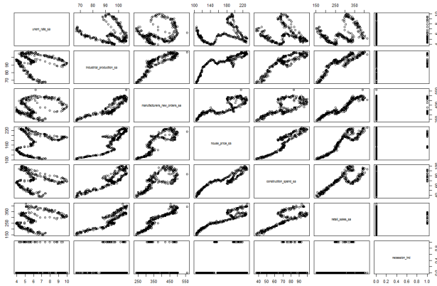
Figure 27: Scatterplot matrix
