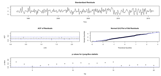
Figure 14: Model 5
