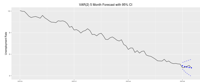
Figure 26: Var(2) Forecast 5 mo
