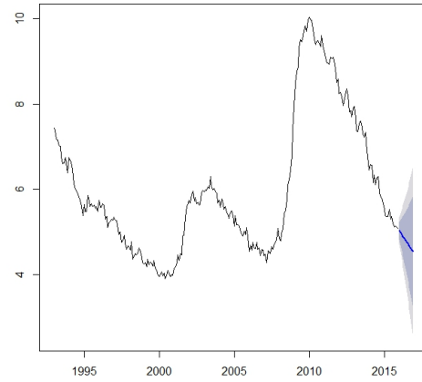
Forecasts from ARIMA(1,2,1)
