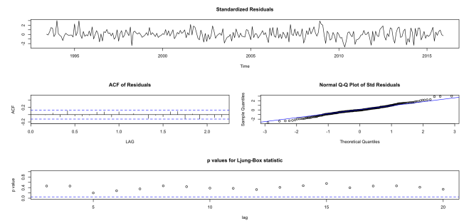
Figure 16: Model 7
