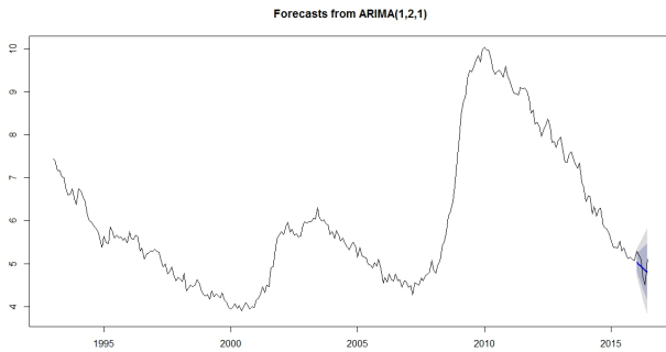
Figure 23: with June 2016
