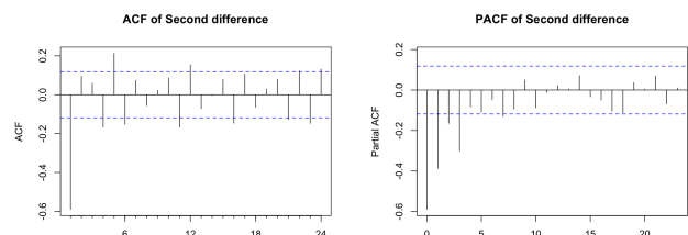
Figure 7: ACF & PACF Plots of Second Differences
