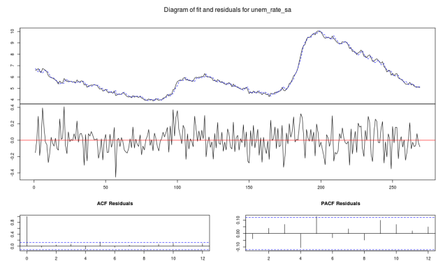
Figure 25: fit and residuals
