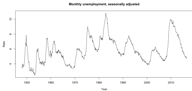
Figure 1: Plot of the original data
