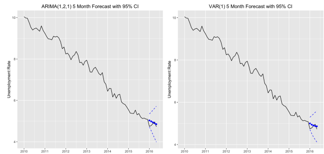
Figure 8: Forecasting with ARIMA and VAR models
