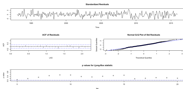
Figure 12: Model 3
