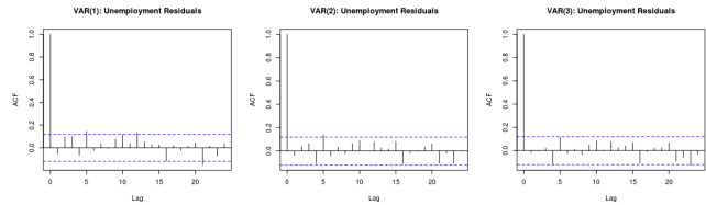
Figure 24: with June 2016
