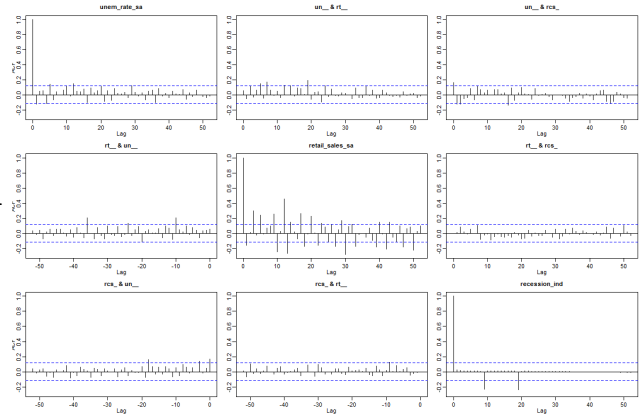
Figure 28: Plots of above
