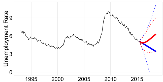
Figure 16: ARIMA and VAR Model comparison of 3 month forecast
