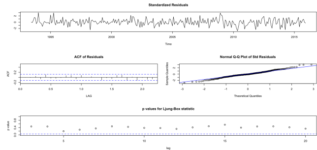
ARIMA(1,2,1) with lagged regressors
