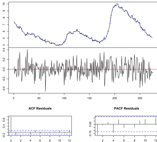
Figure 13: Model 3 fit and residuals for unemployment
