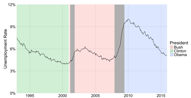
Figure 3: Monthly unemployment, 1993 - 2015
