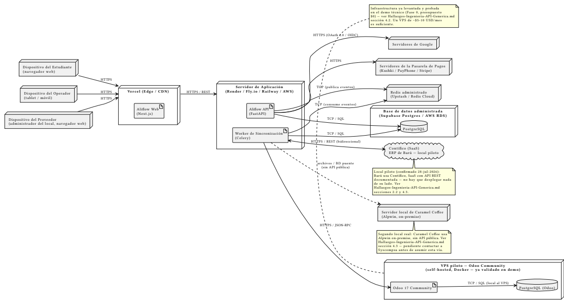
Figure 1: Diagrama de despliegue de Aliflow
