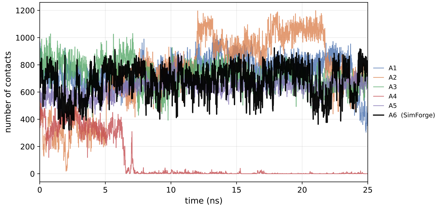
AA (alpha-amylase) - Ligand-active-site contacts (<0.6 nm)
