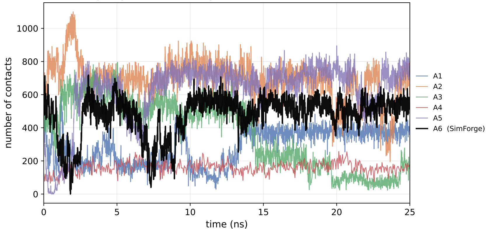
AG (alpha-glucosidase) - Ligand-active-site contacts (<0.6 nm)
