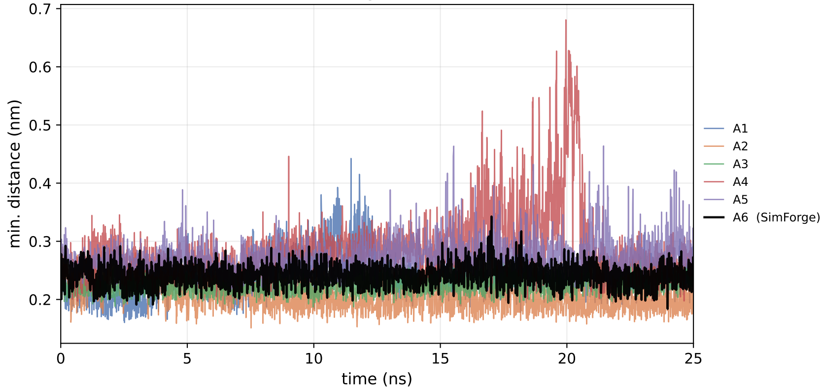
HMG (HMG-CoA reductase) - Ligand-active-site minimum distance
