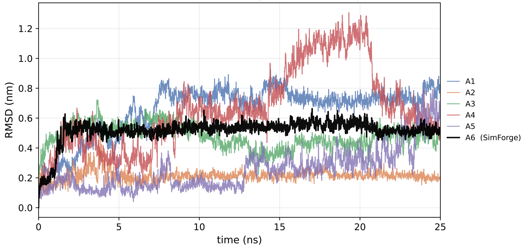
HMG (HMG-CoA reductase) - Ligand RMSD (fit to protein)
