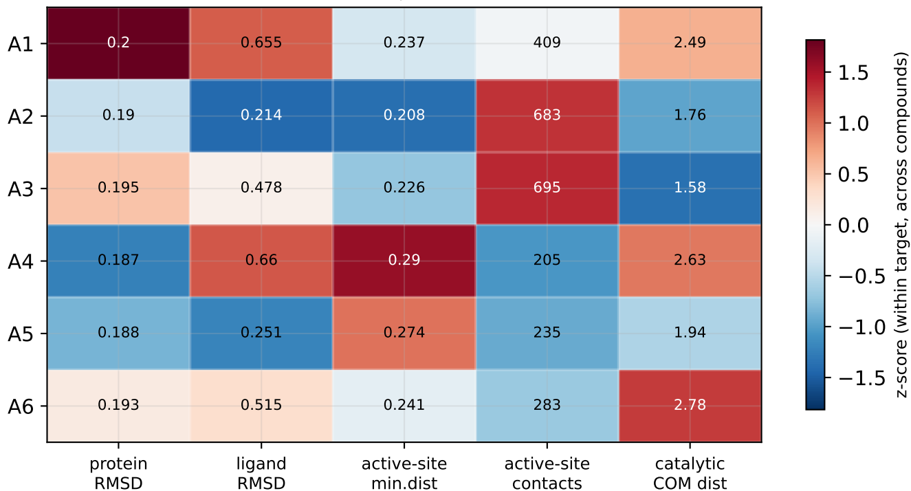
HMG (HMG-CoA reductase) - short-study descriptor profile (cell text = raw mean; colour = per-column z-score across A1-A6)
